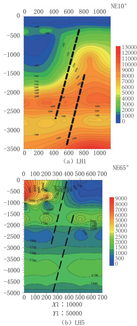
图 4 LH1、LH5 大地电磁测深电阻率等值断面图 [41] Fig.4 Equivalent sections of resistivity of LH1 and LH5 magnetotelluric sounding
