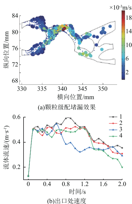
图 7 颗粒级配堵漏效果和出口处流速 Fig.7 Particle size distribution plugging effect diagram and outlet flow velocity
